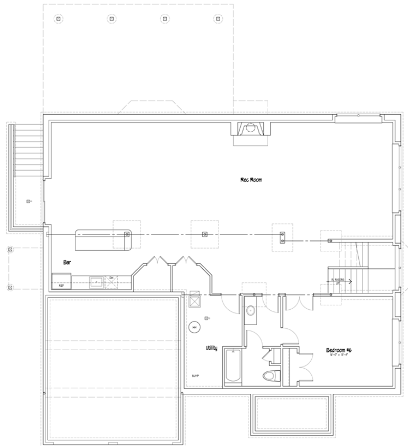
BASEMENT PLAN Scale: 1/4" = 1'-0"
