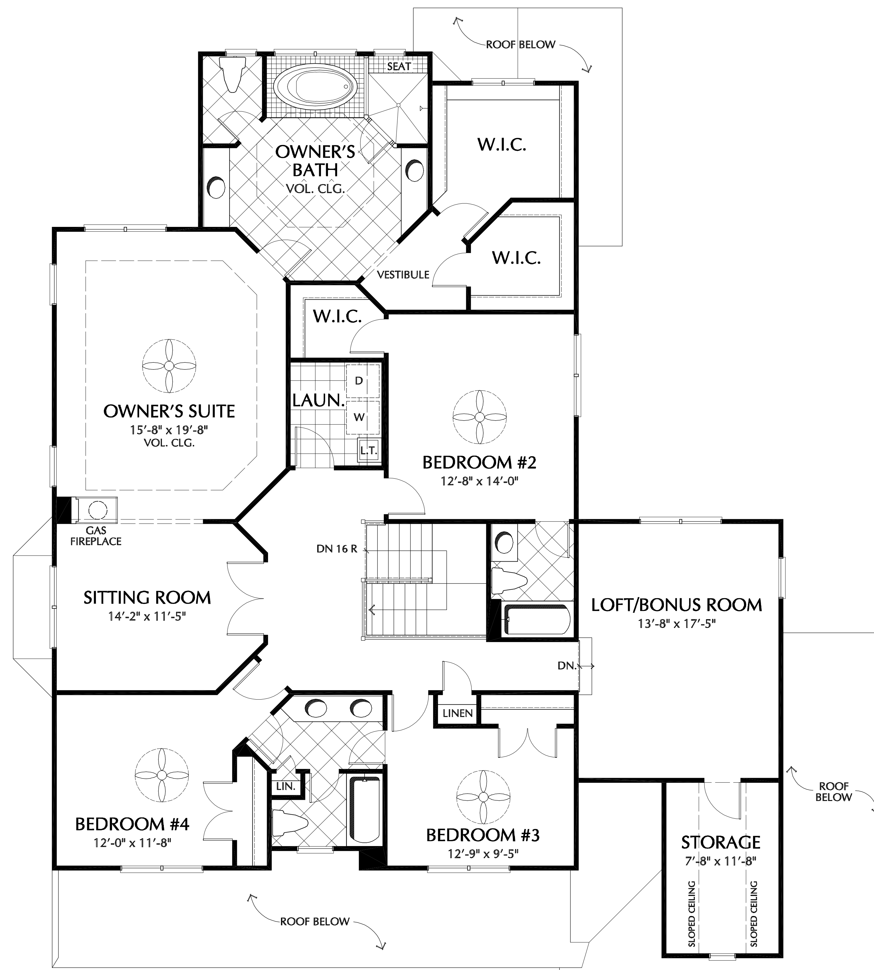
SECOND FLOOR PLAN 2,150 S.F.
